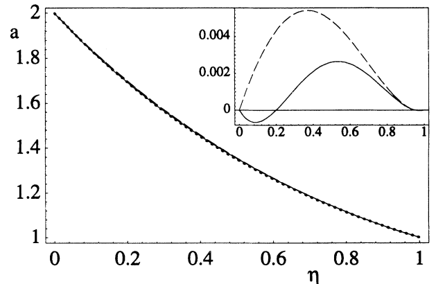
FIG. 5. Behavior of the scaling parameter a versus the packing fraction \eta for hard disks ( D = 2 ): dotted line stands for the BC result [Eq. (16)], solid line for the SPT result [Eq. (17)], and dashed line for the H result [Eq. (18)]. The inset shows the relative differences (a_{\text{SPT}} - a_{\text{BC}})/a_{\text{BC}} (solid line) and (a_{\text{H}} - a_{\text{BC}})/a_{\text{BC}} (dashed line) versus \eta .
